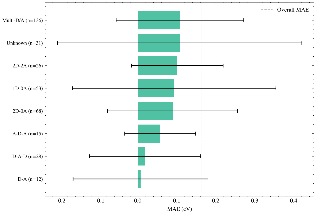
Architecture-Specific Performance with Standard Deviation
